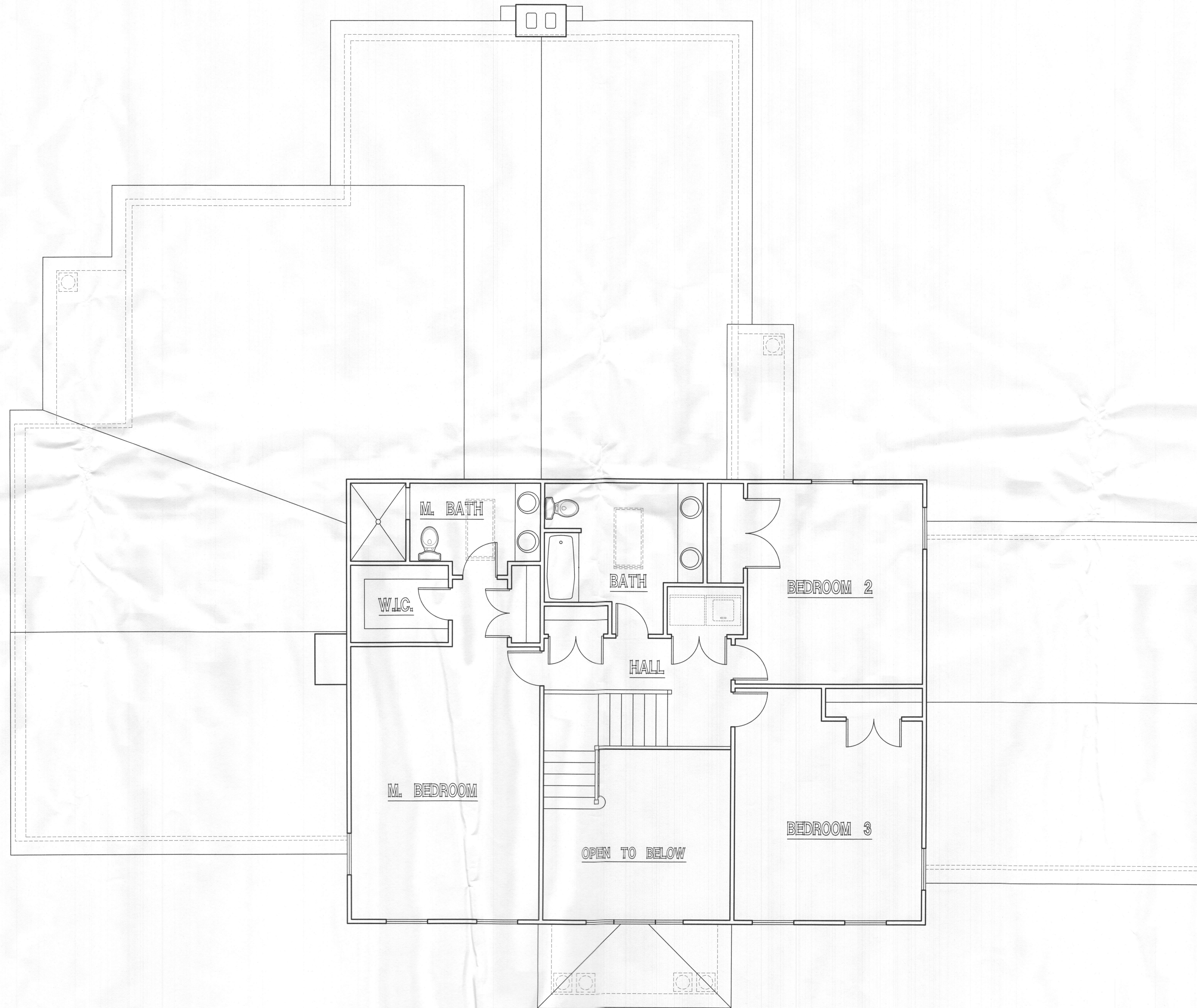
EXIST. SECOND FLOOR PLAN SCALE: 1/4" = 1'-0"
