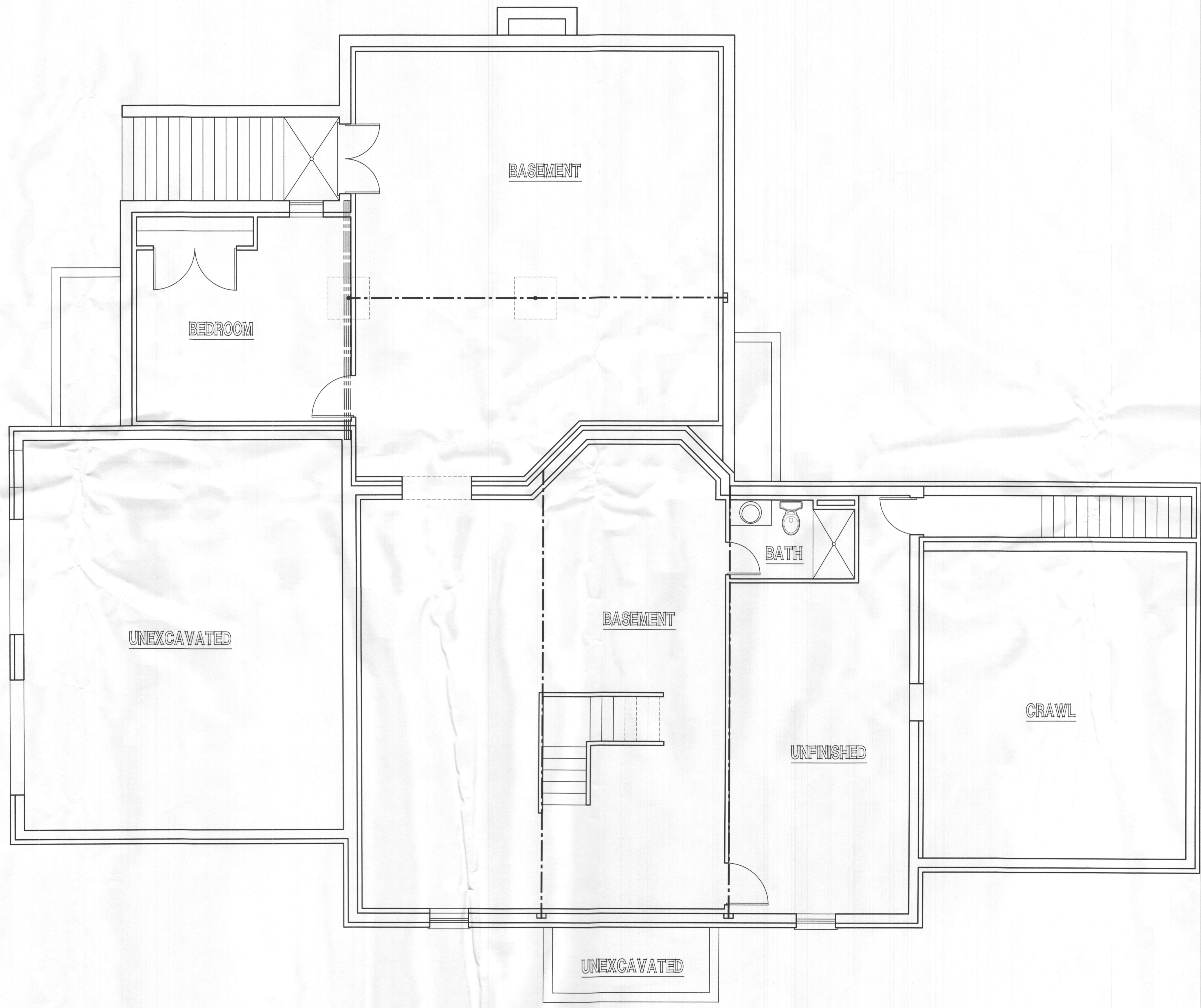
EXIST. FOUNDATION PLAN SCALE: 1/4"=1'-0"
